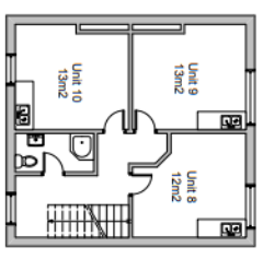
5 Second Floor Scale: 1:100
